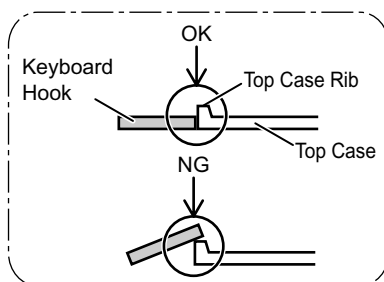
Keyboard hook assembly reference Chart
