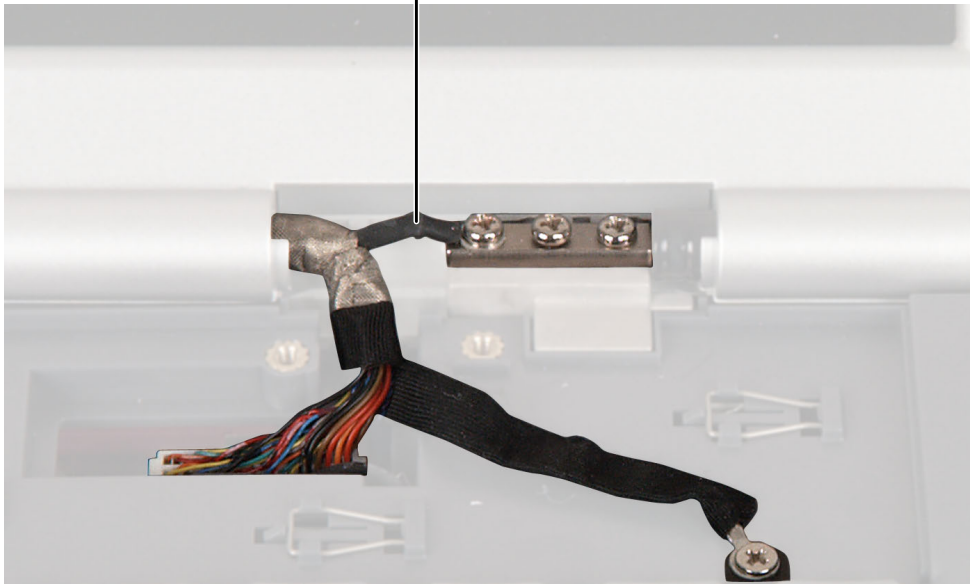
LCD panel ground cable
