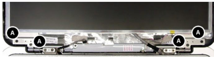
Fig. 21: Releasing the hinges
