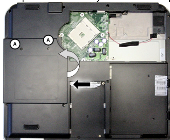
Fig. 10: Removing the CD/DVD drive
