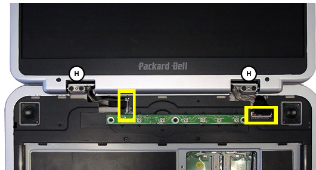
Fig. 18: Removing the LCD assembly
