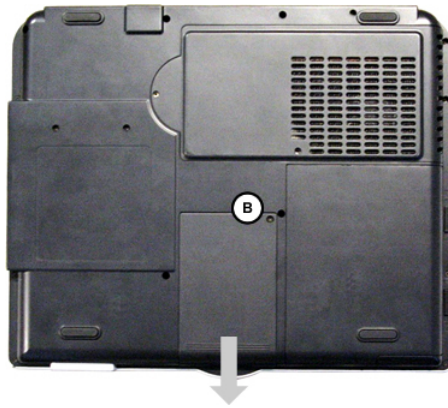
Fig. 6: Removing the HDD cover
