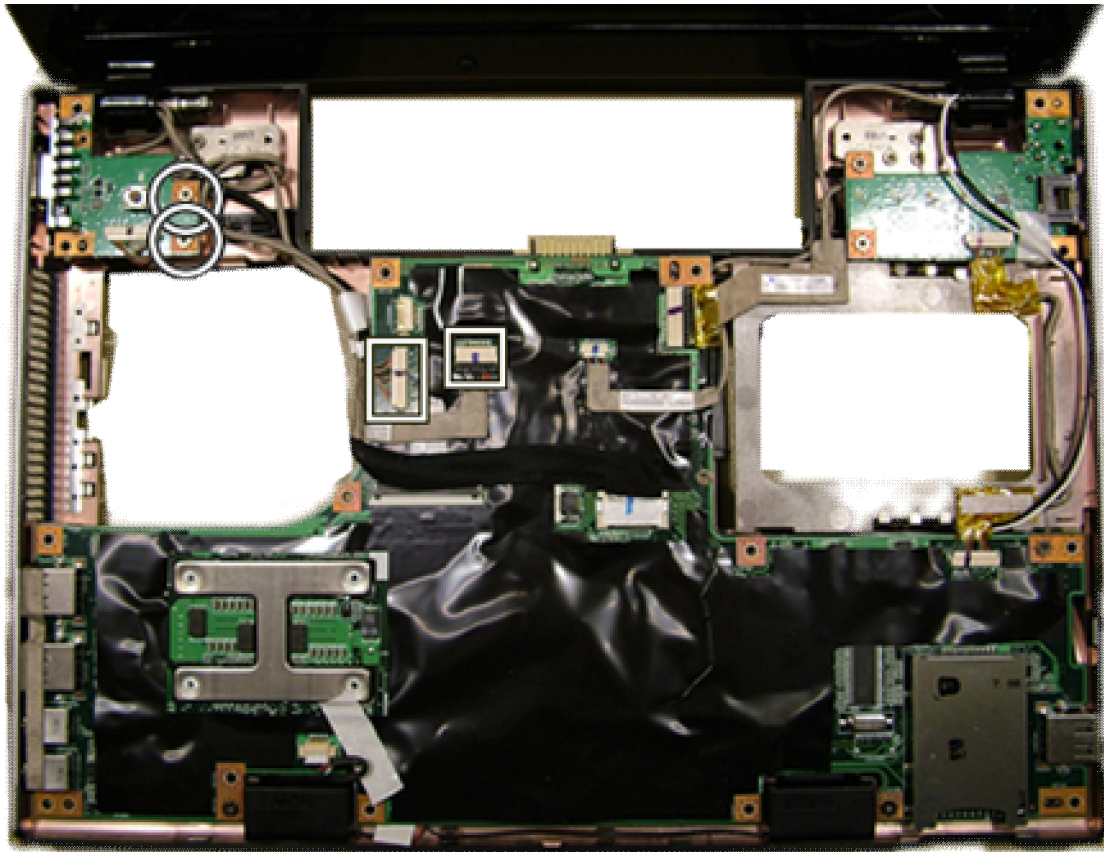
Fig. 20 The connectors and screw for VGA board.
