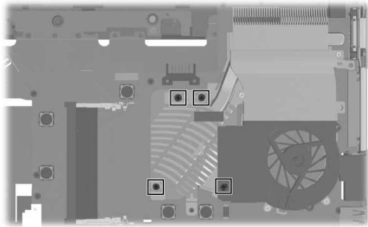
Phillips PM1.5×9.0 Captive Spring-Loaded Shoulder Screw Locations
