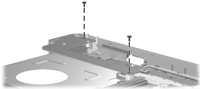
Phillips PM2.0×5.0 Screw Locations
