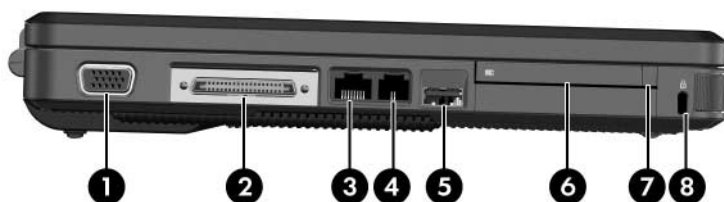
Left-Side Components
