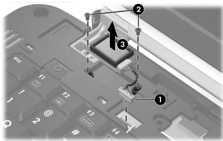
Removing the Bluetooth Board
