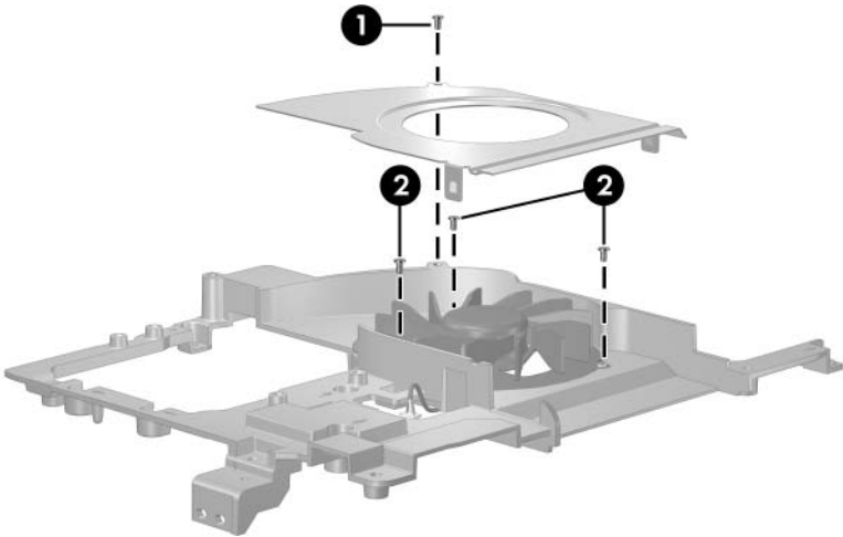
Phillips PM1.5×3.0 Screw Locations
