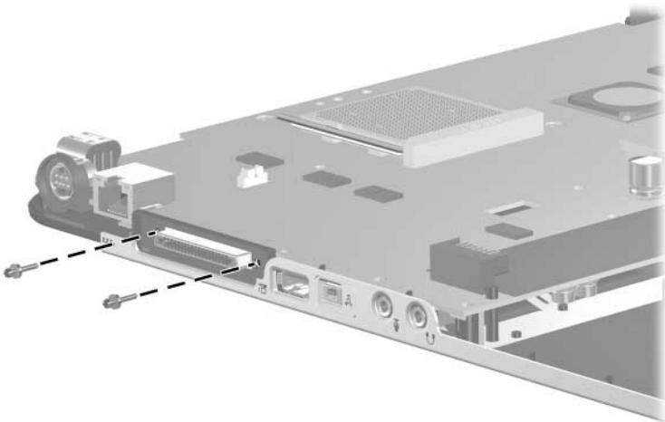
Phillips PM1.5x8.0 Screw Locations
