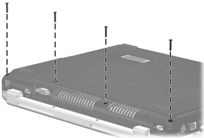
Phillips PM2.0×15.0 Screw Locations
