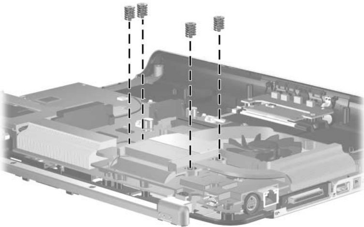
Phillips PM2.0×11.0 Spring-Loaded Shoulder Screw Locations
