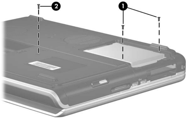
Phillips PM2.0×7.0 Screw Locations
