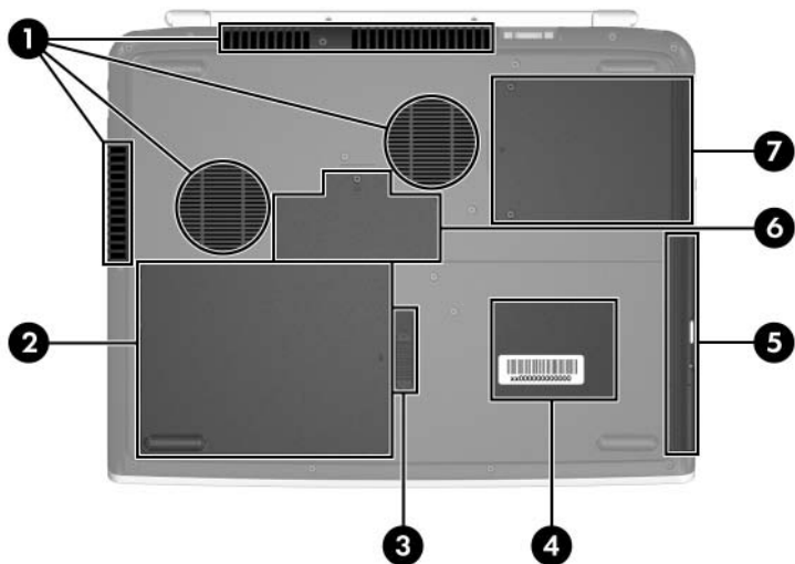
Bottom Components
