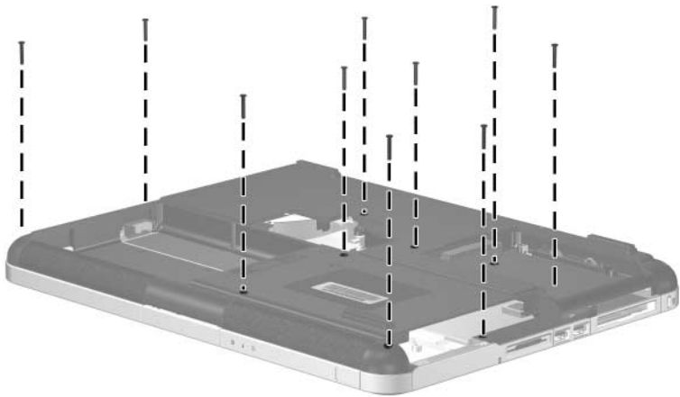
Phillips PM2.0×15.0 Screw Locations
