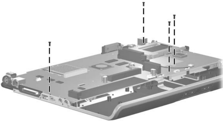
Phillips PM2.0×7.0 Screw Locations
