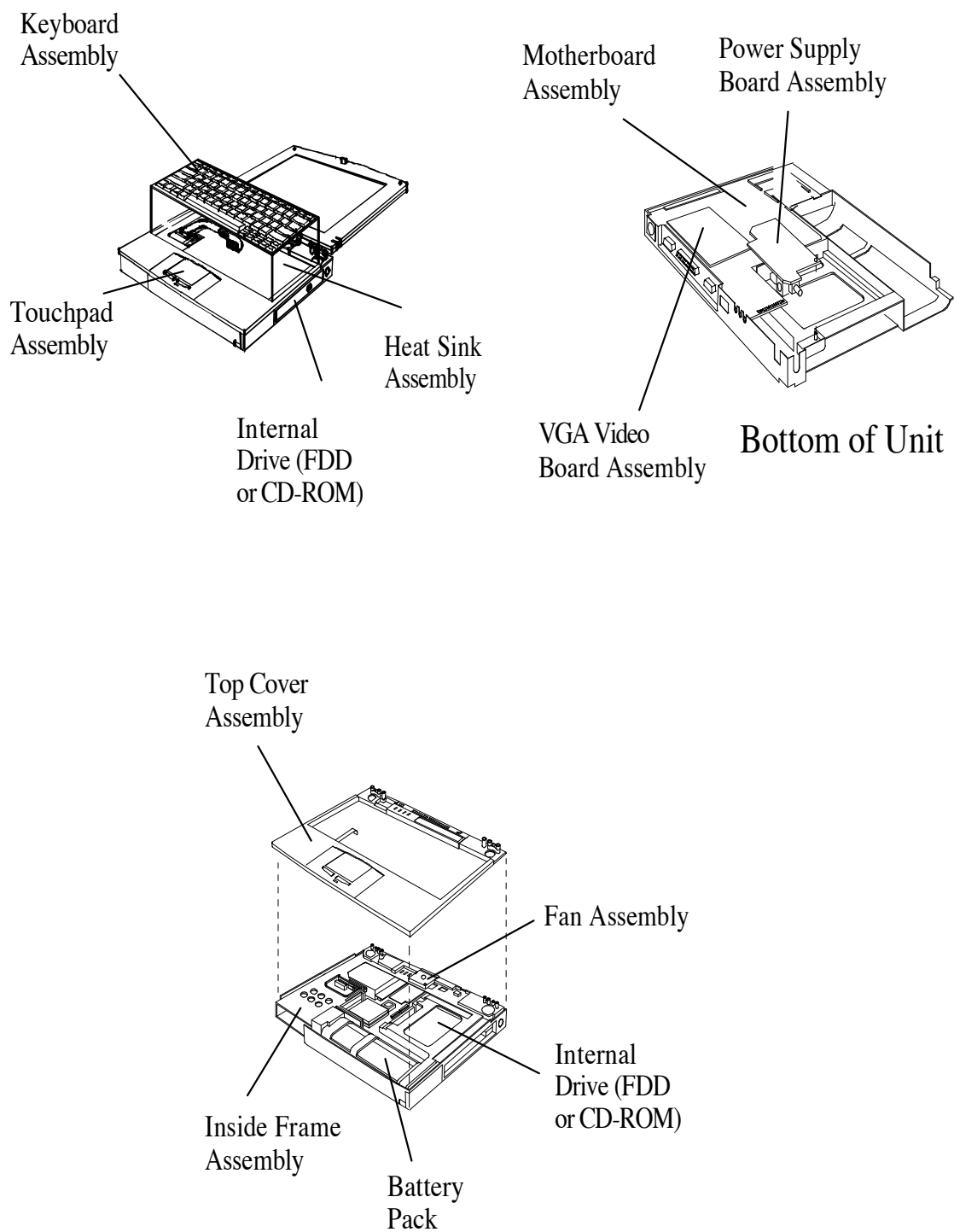
Figure A-3 Base Assembly FRUs
