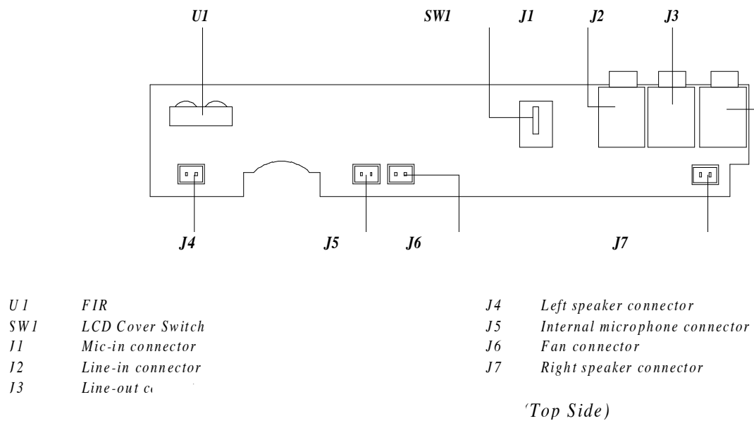
Figure B-8 FIR/Audio Board Jumper Options
